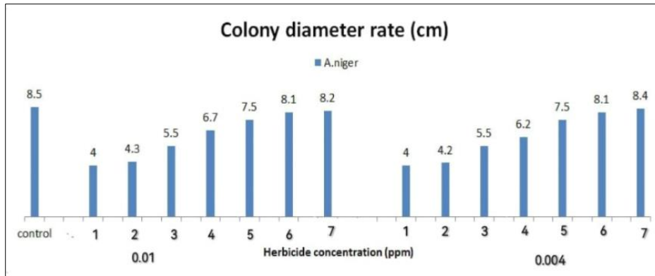
Figure 1 The daily basis effect of Clodinafop-propargyl on A.niger in solid media
