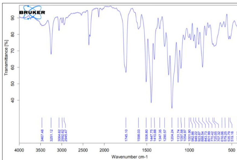
Figure 2 Clodinafop-propargyl (standard)
