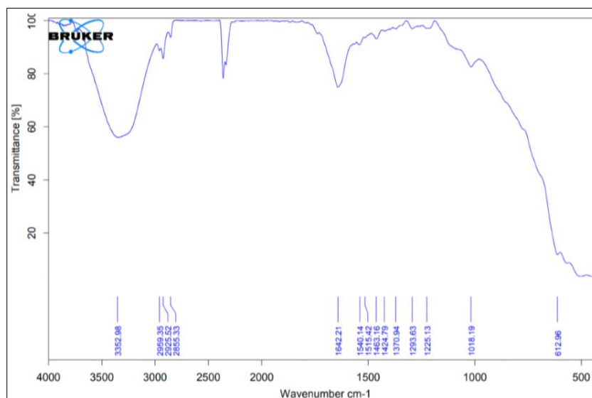
Figure 3 Transformations of Clodinafop-propargyl by A.niger using the (FTIR) spectroscopy
